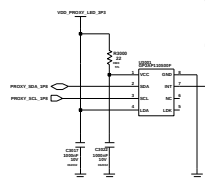
Proxi Sensor
