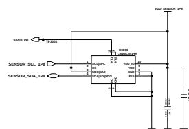
ACC Sensor
