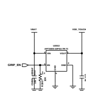
Grip Sensor_LDO
