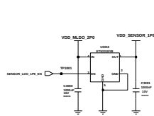
SENSOR 1.8V LDO
