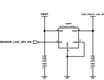
PROXY_SENSOR LDO
