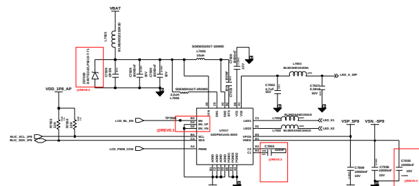
LCD_BL_IC
