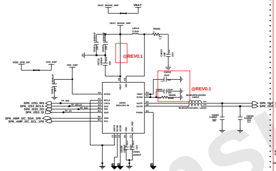
SPK AMP
